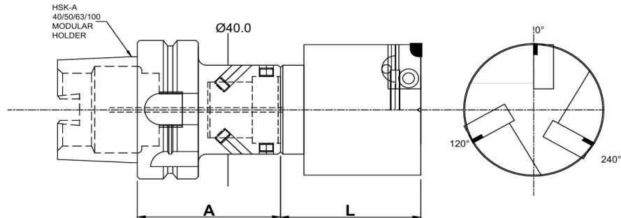
PCD Type Rough Boring Bar (mm)
