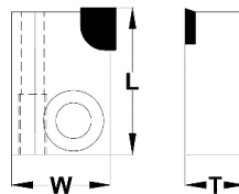
PCD Type Rough Boring Bar Cartridges (mm)
