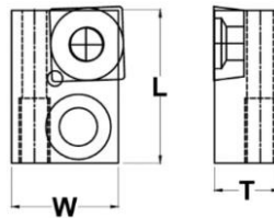
Insert Type Face Fine Boring Bar Cartridge (mm)
