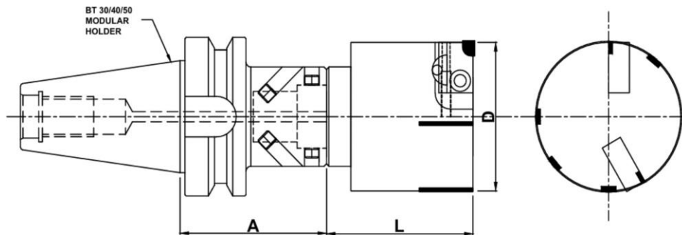
PCD Brezed Type Face Fine Boring Bar (mm)
