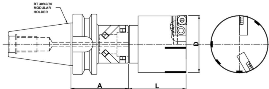
Insert Type Face Fine Boring Bar (mm)
