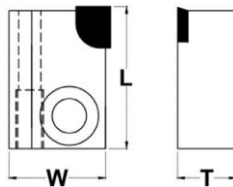
PCD Brezed Type Fine Face Boring Bar Cartridge (mm)
