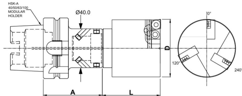
Insert Type Rough Boring Bar (mm)
