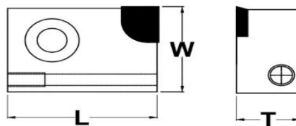
PCD Brezed Type Face Fine Boring Bar Cartridge (mm)
