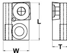
Insert Type Rough Boring Bar Cartridge (mm)
