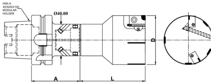
PCD Brezed Type Face Fine Boring Bar (mm)
